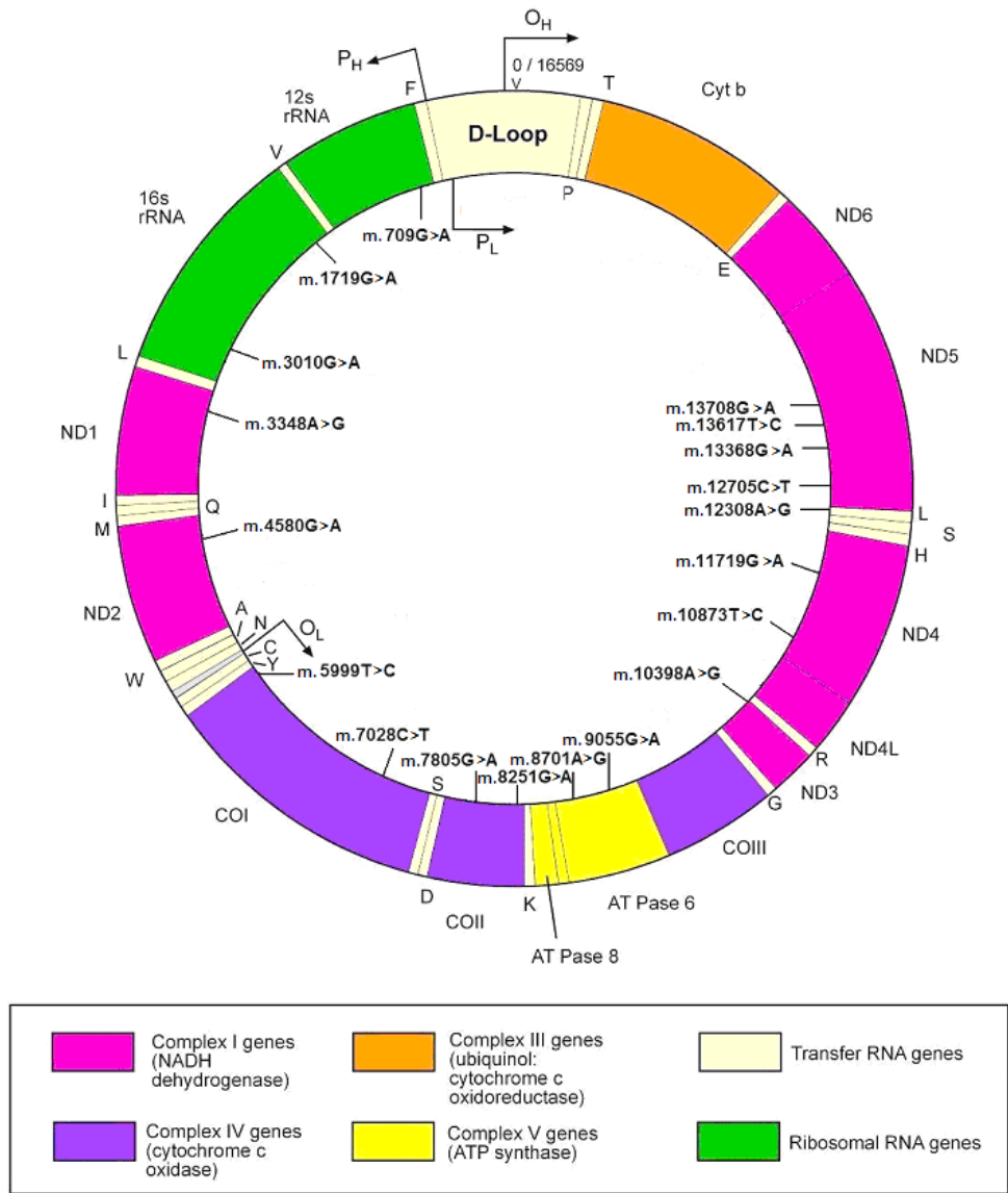
Figure 1 – Location of the mitochondrial genetic markers studied (adapted from Rosa et al. BMC Medical Genetics 2008, 9:57).
